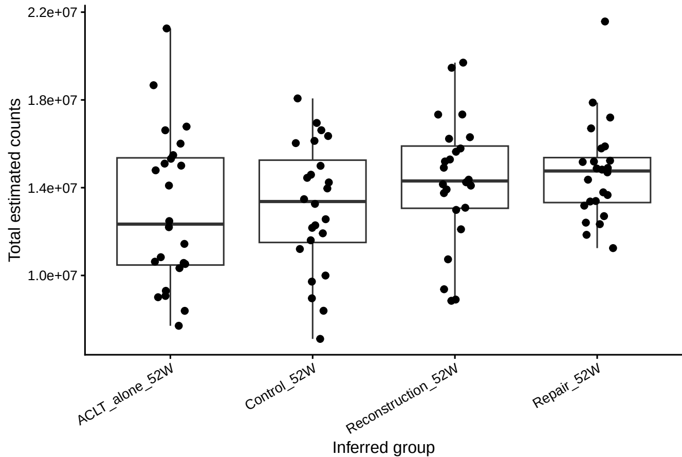
Chronic pig tximport gene-level estimated counts
